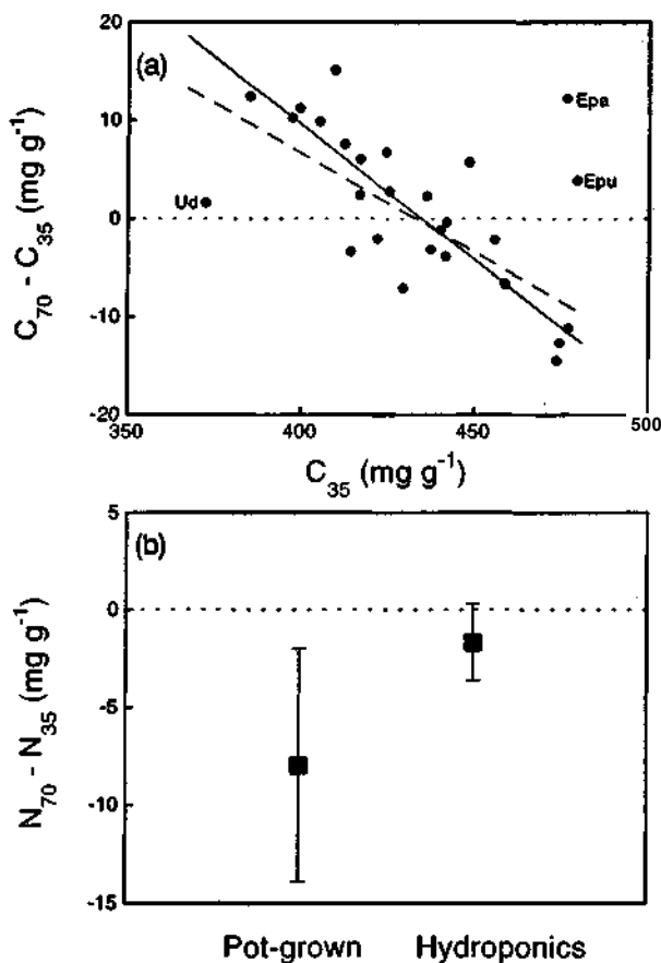
Figure 3. (a) The absolute change in the C concentration (values at 70 Pa - values at 35 Pa) of leaves of 27 species, plotted against the C concentration at control levels of CO 2 . The continuous line is the regression line through the data points ( r^2 = 0.71 , P < 0.001 ), with the exception of three outlying species (Epa: Eucalyptus pauciflora ; Epu: E. pulverulenta ; Ud: Urtica dioica ). The dashed line shows the same relationship, after correction for the TNC in the leaf material. (b) The absolute change in leaf total N concentration (on a TNC-free weight basis) for species grown in pots with soil ( n = 19 ) and in hydroponics ( n = 8 ). Mean values \pm SD are shown.
